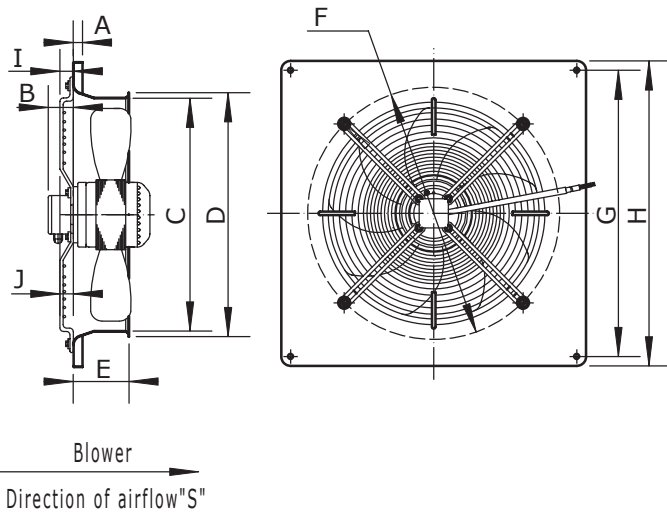
Dimension of Part
