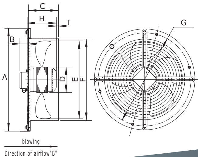
Dimension of Part
